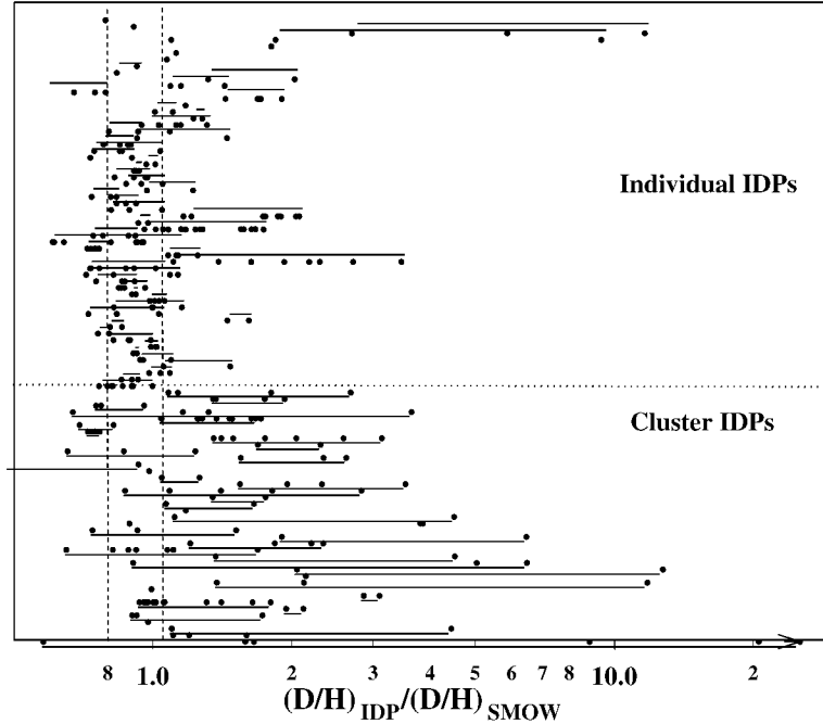
Figure 1. Comparison of D/H ratios of cluster and individual IDPs relative to the terrestrial standard mean ocean water (SMOW). The D/H ratios of different fragments of each IDP are shown as points, where the lines denote the range of values observed in each particle. The particle with the highest D/H ratio in the figure (Dragonfly) reaches a D/H ratio of 50 times solar, estimated by ion imaging (not shown). The range of D/H values observed among terrestrial rocks is shown by the vertical dashed lines.
